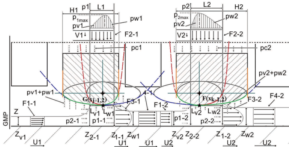
Fig. 1. Schematic representation of asymmetric geometry of parabolic and elliptical sliding surfaces, as well as velocity and pressure fields at the starting and separating points of the oil film for the lower and upper sealing rings where: \star – W_{j,k1-2} vertex coordinates of the parabolas and ellipses defining the given asymmetric shape of the sliding surface, \blacklozenge – coordinates of the ellipses common center, green line – function expressing the asymmetrical shape of the sealing rings sliding surfaces
