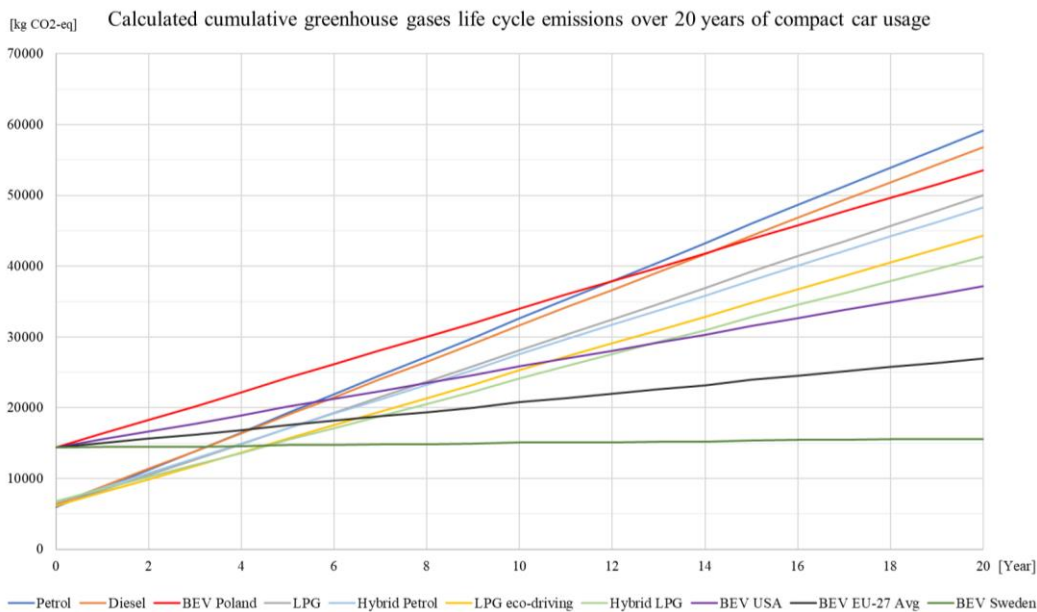
Fig. 2. Calculated cumulative greenhouse gases life cycle emissions over 20 years of compact car usage
