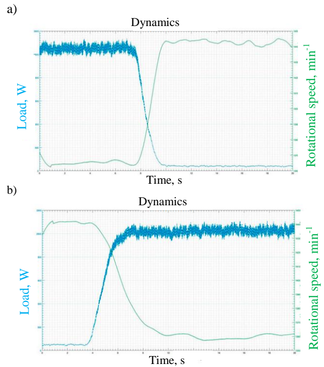
Fig. 5. Time courses of the load and crankshaft rotational speed of the research engine in the acceleration (a) and deceleration (b) processes [6]
