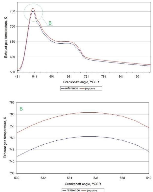
Fig. 4. Runs of changes in the temperature of the exhaust gas T_{exh} value for the crankshaft rotation angle, for portion of the engine operating cycle and for the region of existence of the peak value of the flue gas temperature, obtained by numerical simulation in the DIESEL-RK program for two values of injector opening pressure p_{inj} [23]
