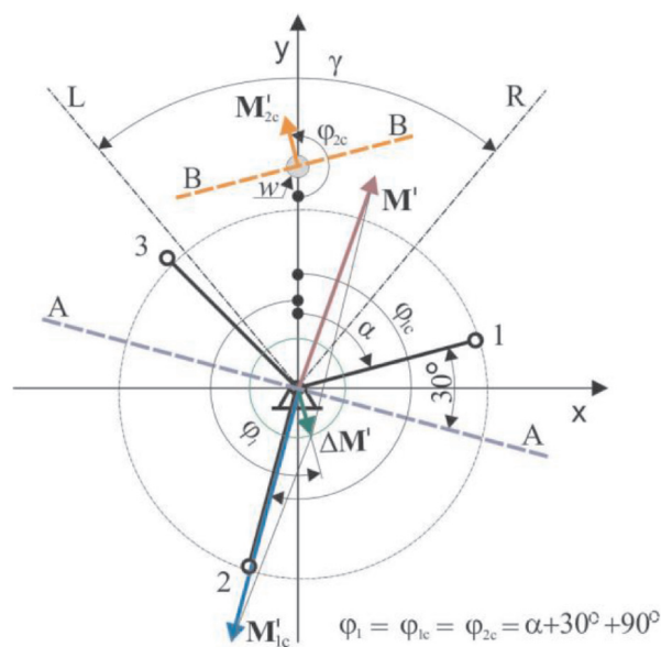
Fig. 11. Vector system of moments for \gamma = 80^\circ , \alpha = 75^\circ
