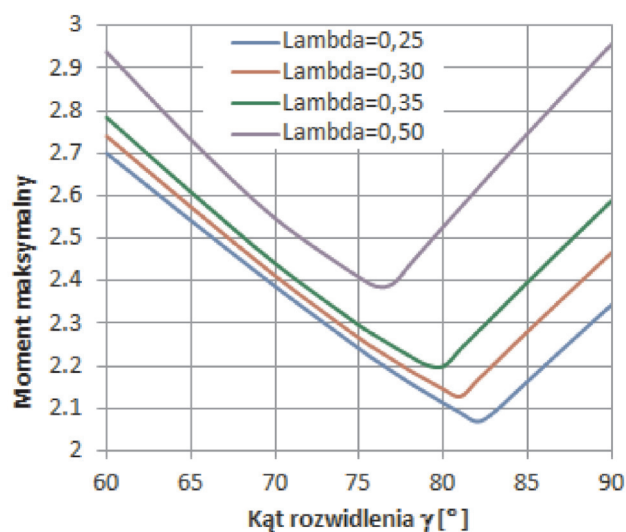
Fig. 4. Plots of the maximum moment of the inertia forces for \gamma \in (60^\circ - 90^\circ) and different values of \lambda
