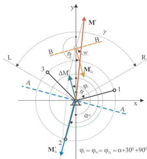
Fig. 12. Vector system of moments for \gamma = 120^\circ , \alpha = 75^\circ
