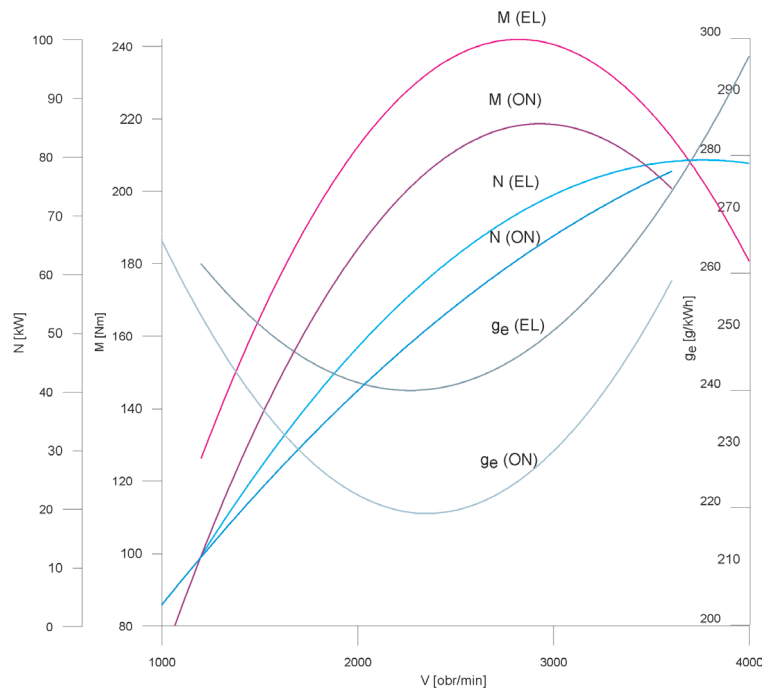
Fig. 2. Comparison of 4CT90 engine full load characteristics fuelled with diesel fuel and EL [4]
