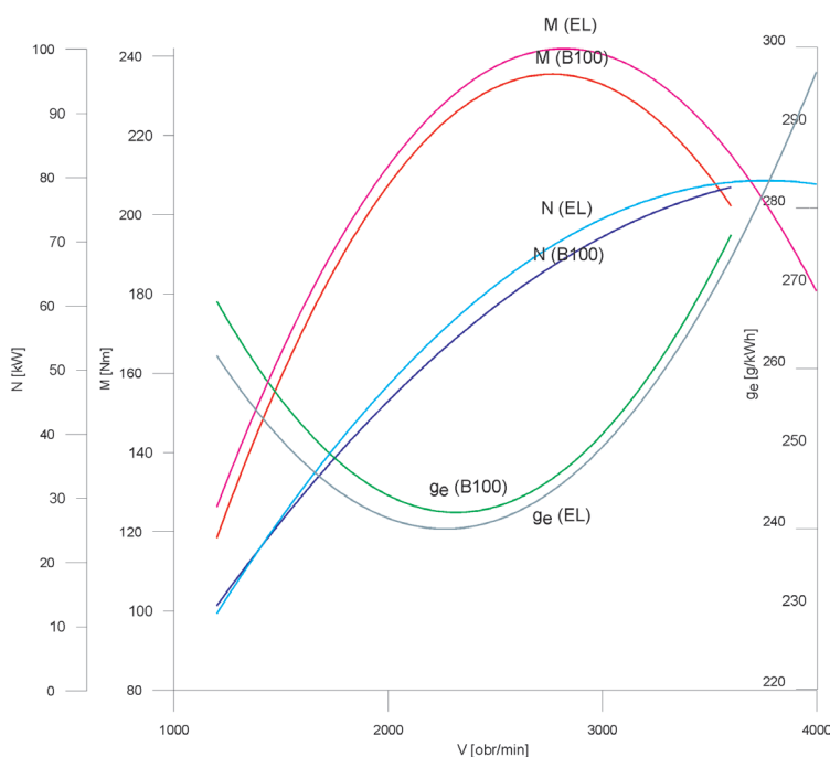
Fig. 3. Comparison of 1.4D-4D engine full load characteristics fuelled with EL and B100 [4]
