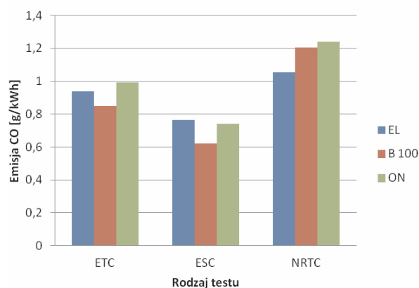
Fig. 7. CO emissions in ETC, ESC and NRTC cycles, engine fuelled with EL, B100 and Diesel fuel
