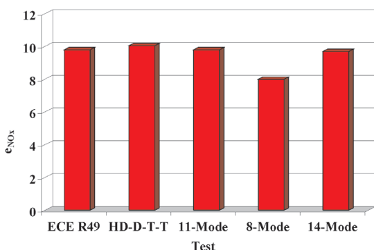
Fig. 6. Specific brake emission of nitric oxides in tests determined in accordance with the criterion of equality of average effective power
