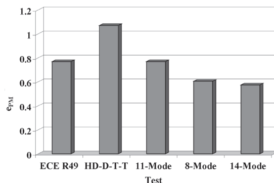
Fig. 7. Specific brake emission of particulate matter in tests determined in accordance with the criterion of equality of average effective power
