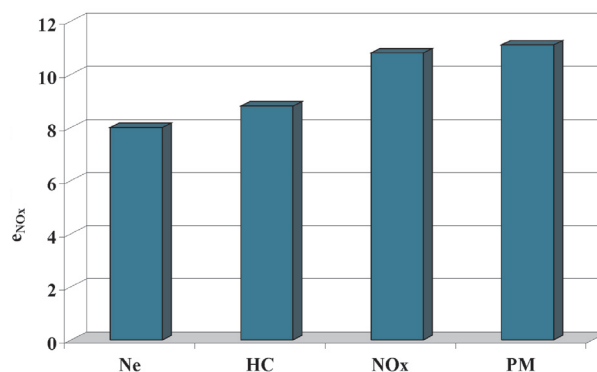
Fig. 9. Specific brake emission of nitric oxides in 8-mode tests determined in accordance with various criteria of similarity
