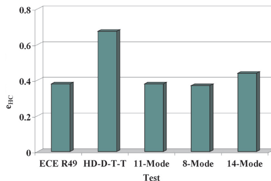
Fig. 5. Specific brake emission of hydrocarbons in tests determined in accordance with the criterion of equality of average effective power
