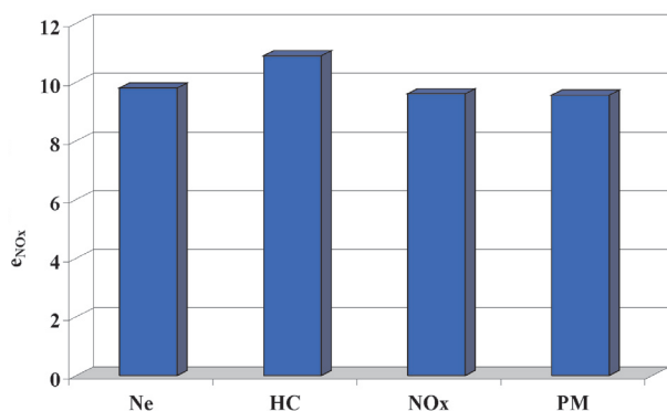
Fig. 8. Specific brake emission of nitric oxides in 11-mode tests determined in accordance with various criteria of similarity
