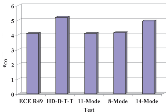
Fig. 4. Specific brake emission of carbon monoxide in tests determined in accordance with the criterion of equality of average effective power
