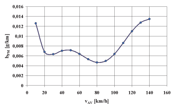
Fig. 4. The dependence of specific road emission of particulate matter b_{PM} from passenger vehicle engines on the average speed v_{AV}
