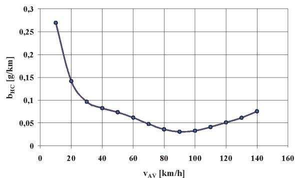
Fig. 2. The dependence of specific road emission of hydrocarbons b_{HC} from passenger vehicle engines on the average speed v_{AV}
