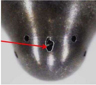
Fig. 3. Destroyed marine engine fuel nozzle due to destructive effects of catalytic fines [1]
