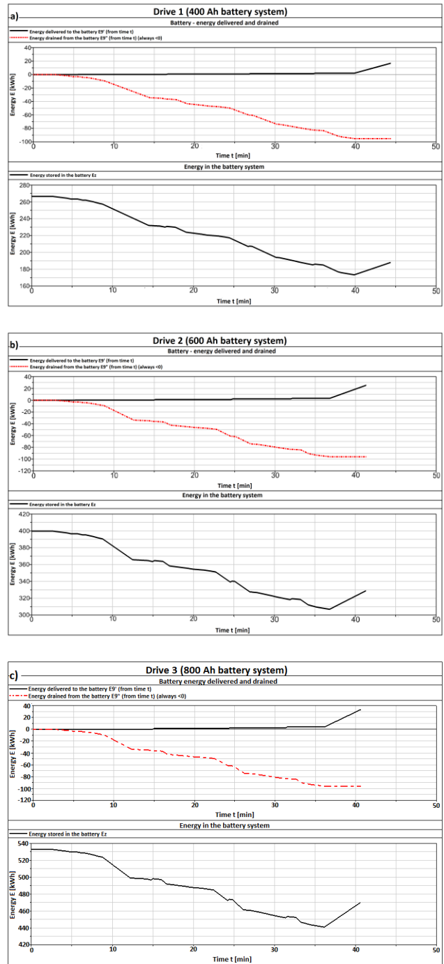
Fig. 4. Energy storage system state of charge and Energy depletion in the simulation drive for each vehicle variant: a) drive 1, b) drive 2, c) drive 3
