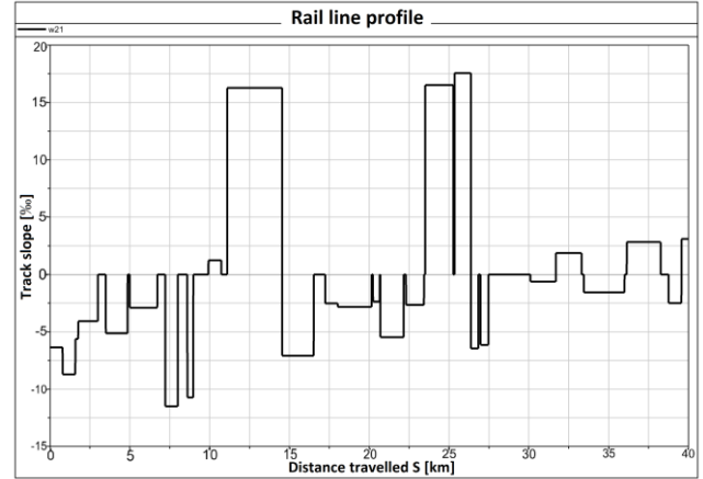
Fig. 1. Track incline profile for the test route
