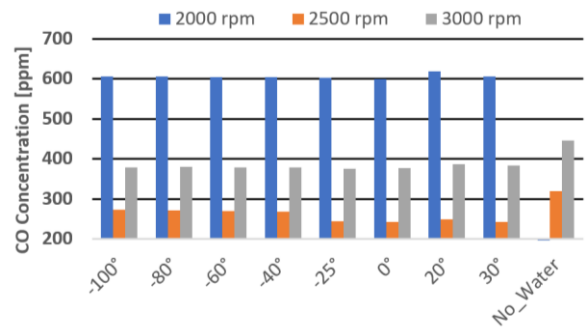
Fig. 27. CO concentration in ppm for the cycle without water injection and for each water injection angle for the W/F ratio of 0.15
