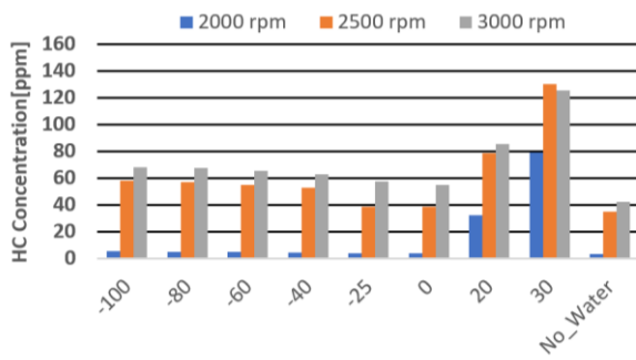
Fig. 33. HC concentration in ppm for the cycle without water injection and for each water injection angle for the W/F ratio of 0.2
