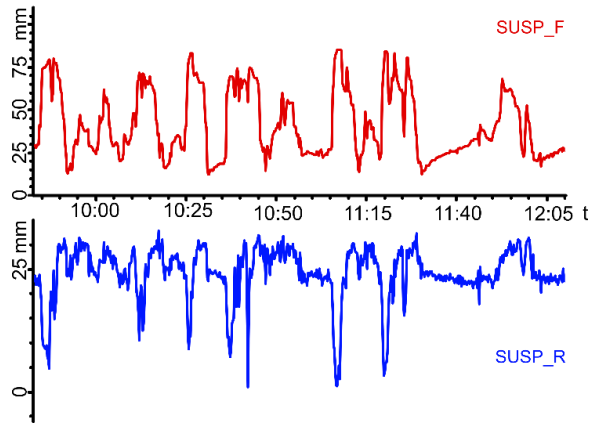
Fig. 7. Suspension plot, illustrating suspension behavior and dynamics across different sections of the circuit at second lap
