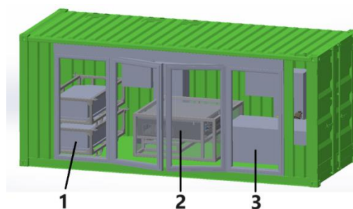
Fig. 6. Power electronics module: 1 – traction batteries, 2 – traction container, 3 – traction motor
