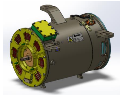
Fig. 9. Traction motor built in a container with power electronics components
