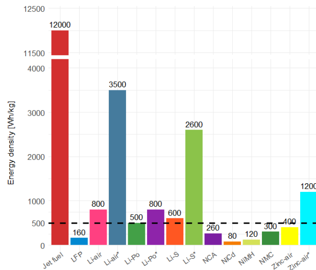
Fig. 4. Comparison of energy densities of different types of rechargeable batteries | * maximum theoretical energy density of a given type of rechargeable battery
