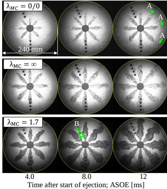
Fig. 5. Ejection behaviours of torch flames under different MC in-chamber gas conditions; \lambda_{MC} = 0/0 : N_2 (top), \lambda_{MC} = \infty : air (middle), and \lambda_{MC} = 1.7 : premixture of CH_4 /air (bottom) with reference PC1 ( N_o = 8 , D_o = \varnothing 3.5 mm)
