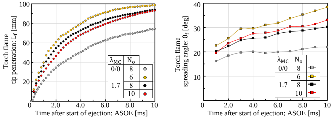
Fig. 7. Effects of number of PC orifices; N_o on torch flame penetration: L_f and its spreading angle: \theta_f by PC2 ( N_o = 6 , D_o = \varnothing 4.0 mm), PC1 (8, \varnothing 3.5 mm), and PC3 (10, \varnothing 3.1 mm) respectively with ca. same A_o
