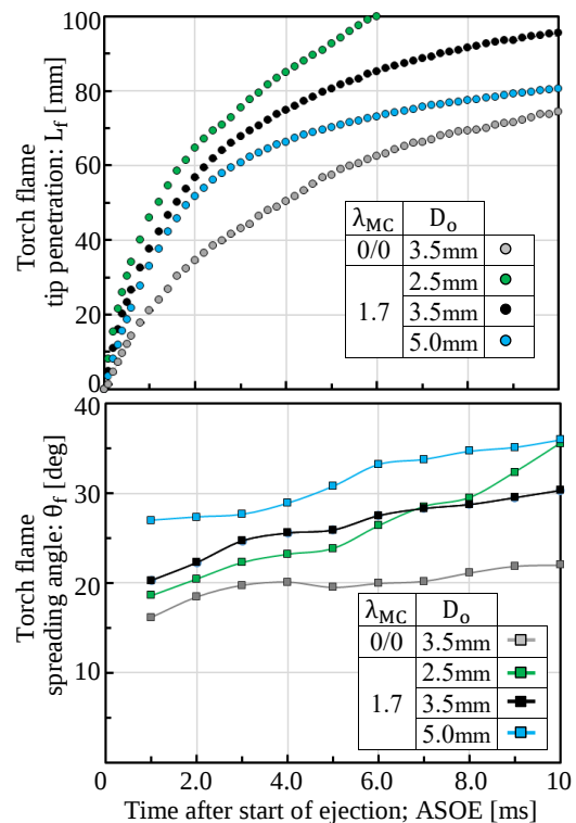
Fig. 10. Effects of diameter of PC orifices; D_o on torch flame penetration: L_f and spreading angle: \theta_f by PC4 ( D_o = \varnothing 2.5 mm), PC1 ( \varnothing 3.5 mm), and PC5 ( \varnothing 5.0 mm)
