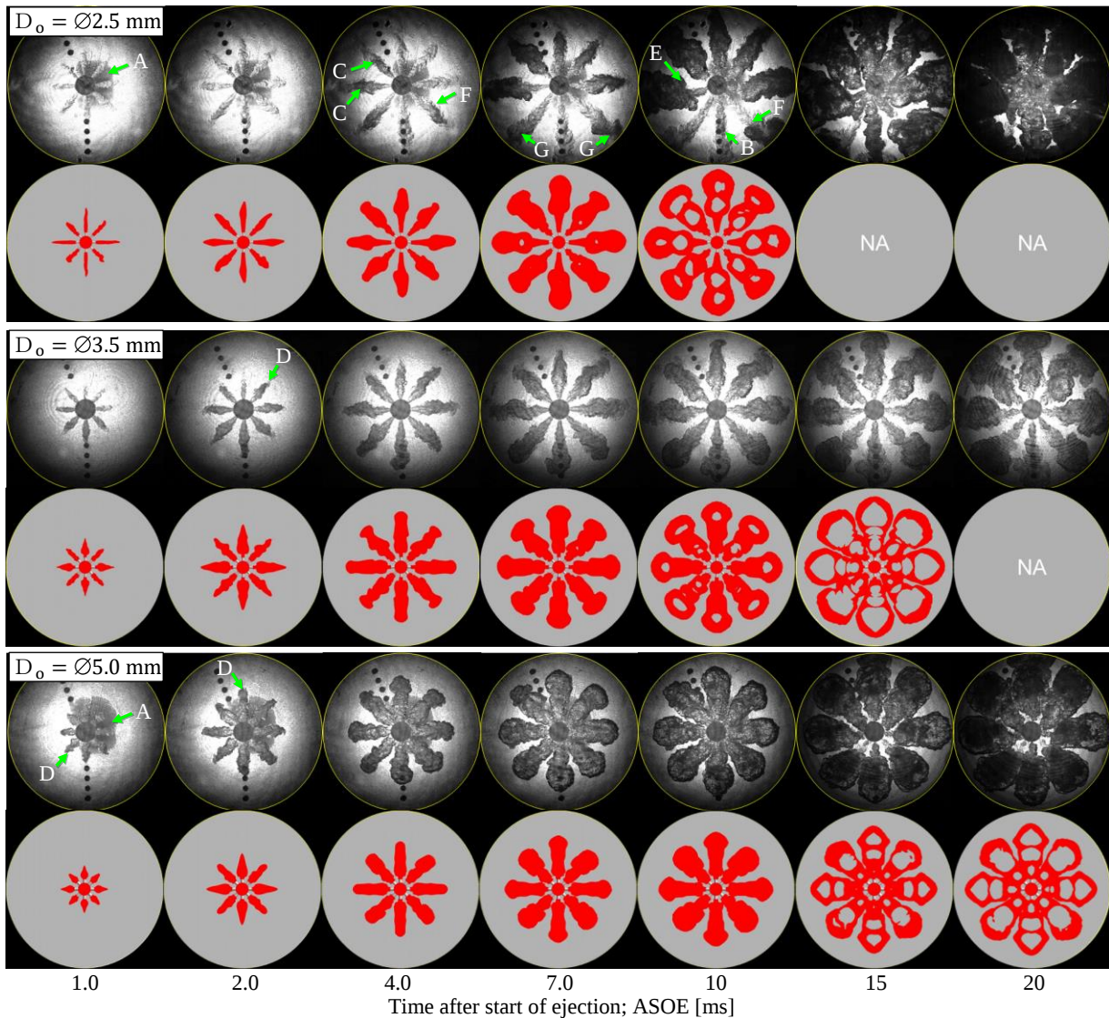
Fig. 11. Effects of diameter of orifices; D_o on ejection behaviour of torch flame by PC4 ( D_o = \varnothing 2.5 mm), PC1 ( \varnothing 3.5 mm), and PC5 ( \varnothing 5.0 mm). Shadowgraph images (upper row of each island) and simulation results (lower row of each island)
