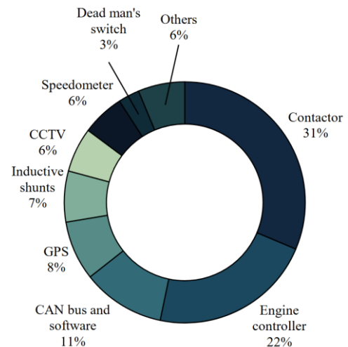
Fig. 4. Failure structure of the electrical equipment
