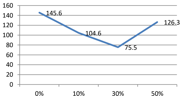
Fig. 3. Amount of solid particles depending on ethanol content in fuel
