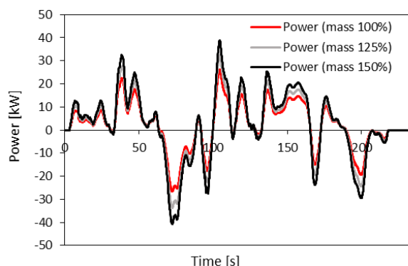
Fig. 15. Influence of vehicle mass on mechanical power supplied/received by the drive system for route 4
