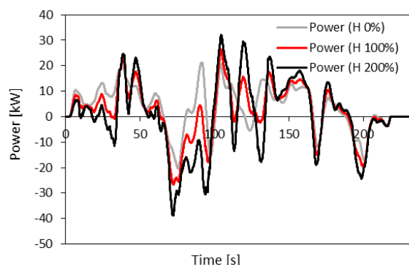
Fig. 16. Influence of road gradient (height multiplication) on mechanical power supplied/received by the drive system for route 4
