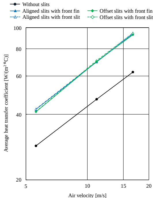
Fig. 8. Average heat transfer coefficient vs. air velocity
