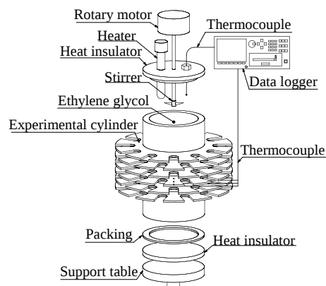
Fig. 3. Experimental apparatus
