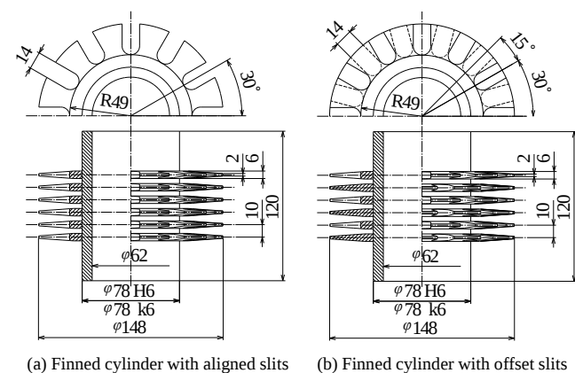
Fig. 1. Experimental finned cylinder with slits
