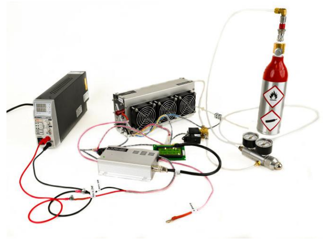
Fig. 6. Object of the research – Horizon-300W fuel cell [21]
