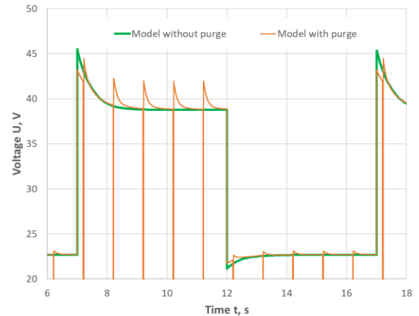
Fig. 13. Voltage simulation with and without active cleaning module during changed load condition
