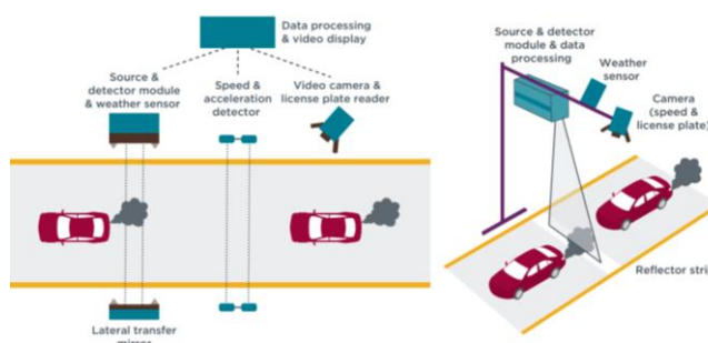
Fig. 6. Open path measurement scheme: a) configuration used at intersections, b) top-down detection system [8]
