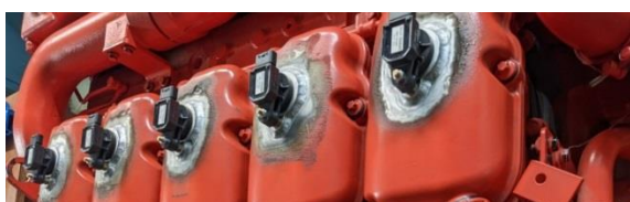
Fig. 14. Arrangement of ignition modules in the engine
