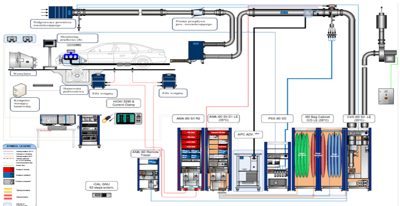
Fig. 1. Laboratory 1 equipment and setup schematic [1]
