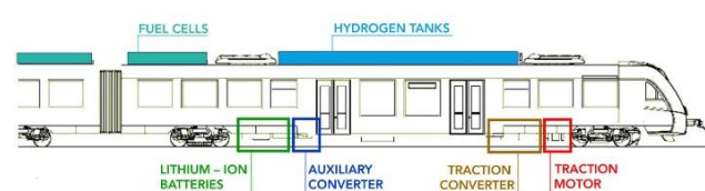
Fig. 1. A trainset manufactured by Alstom, using a hydrogen drive system [26]
