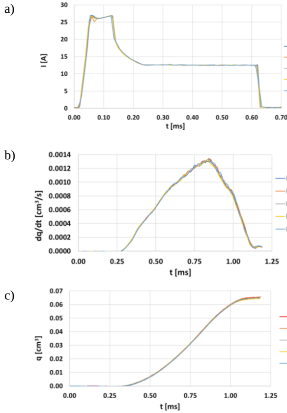
Fig. 5 Injection runs and characteristics obtained from a series of measurements under idle running conditions: a) run and intensity of the current supplying the injector solenoid valve coil, b) fuel injection runs and characteristics in differential form, c) fuel injection runs and characteristics in integral form
