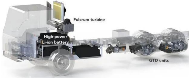
Fig. 1. Application of a turbine as a generator in heavy goods vehicles [14]
