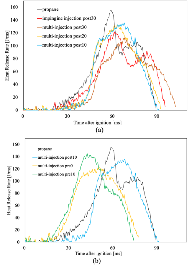
Fig. 7. Heat release rate (HRR) of n-hexadecane under different injection strategies: a) post-injection strategies (impinging and multi-injection); b) pre-injection strategies (multi-injection)
