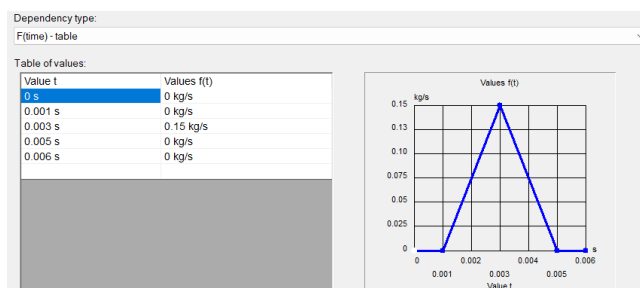
Fig. 5. Injection profile A
