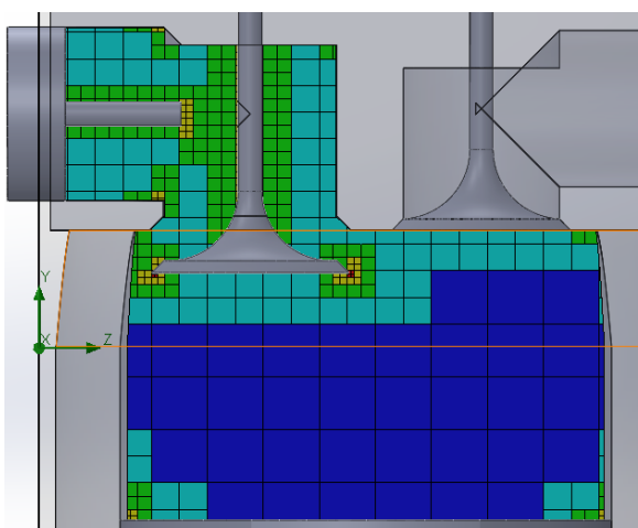
Fig. 3. Yamaha EH65 engine basic mesh model
