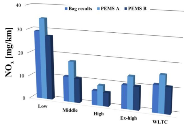
Fig. 11. \text{NO}_x specific distance emission in WLTC test in 23°C from cold start engine in laboratory 2
