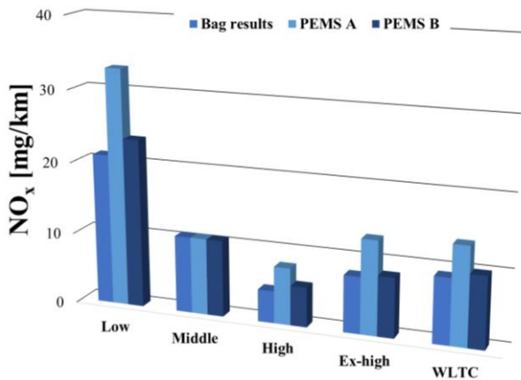
Fig. 9. \text{NO}_x specific distance emission in WLTC test in 14°C from cold start engine in laboratory 2
