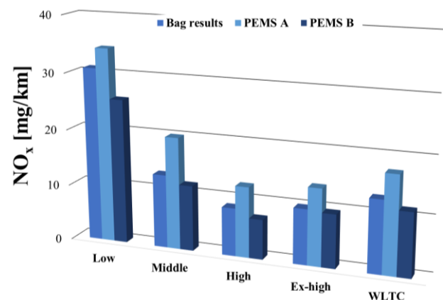
Fig. 12. \text{NO}_x specific distance emission in WLTC test in 23°C from hot start engine in laboratory 2
