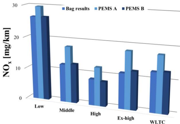
Fig. 10. \text{NO}_x specific distance emission in WLTC test at 14°C from the hot start engine in laboratory 2
