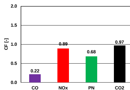
Fig. 11. Emission index determined during on-road tests for the gasoline engine vehicle
