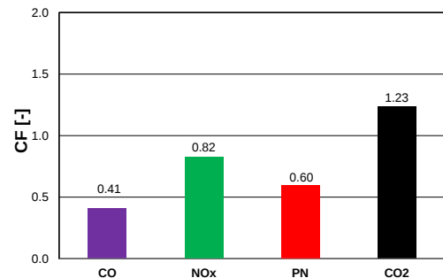
Fig. 13. On-road emissions of exhaust gas constituents determined during tests for the diesel engine vehicle
