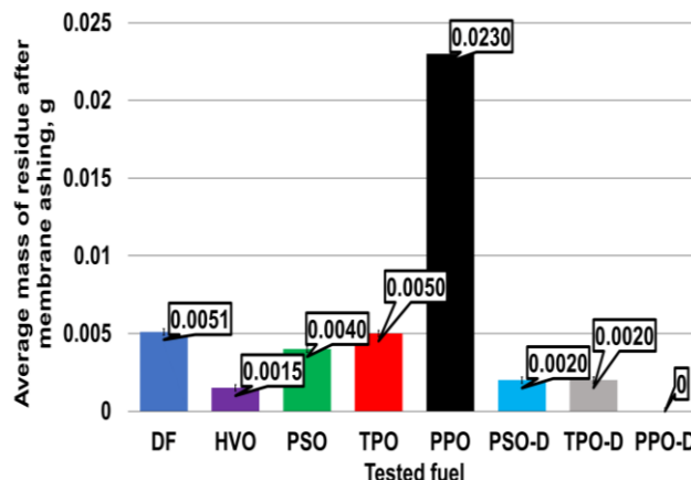
Fig. 8. Average mass of residue after filtration membrane ashing followed by high-temperature drying
