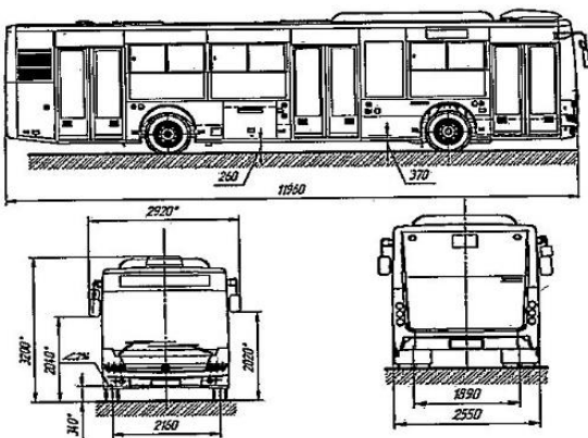
Fig. 9. City bus technical data of the sample bus network voltage 500 V; battery 119 cells of 4.2 V, R = 2.28 Ω; inverter; traction motor 170 kW (continuous power) [7]
