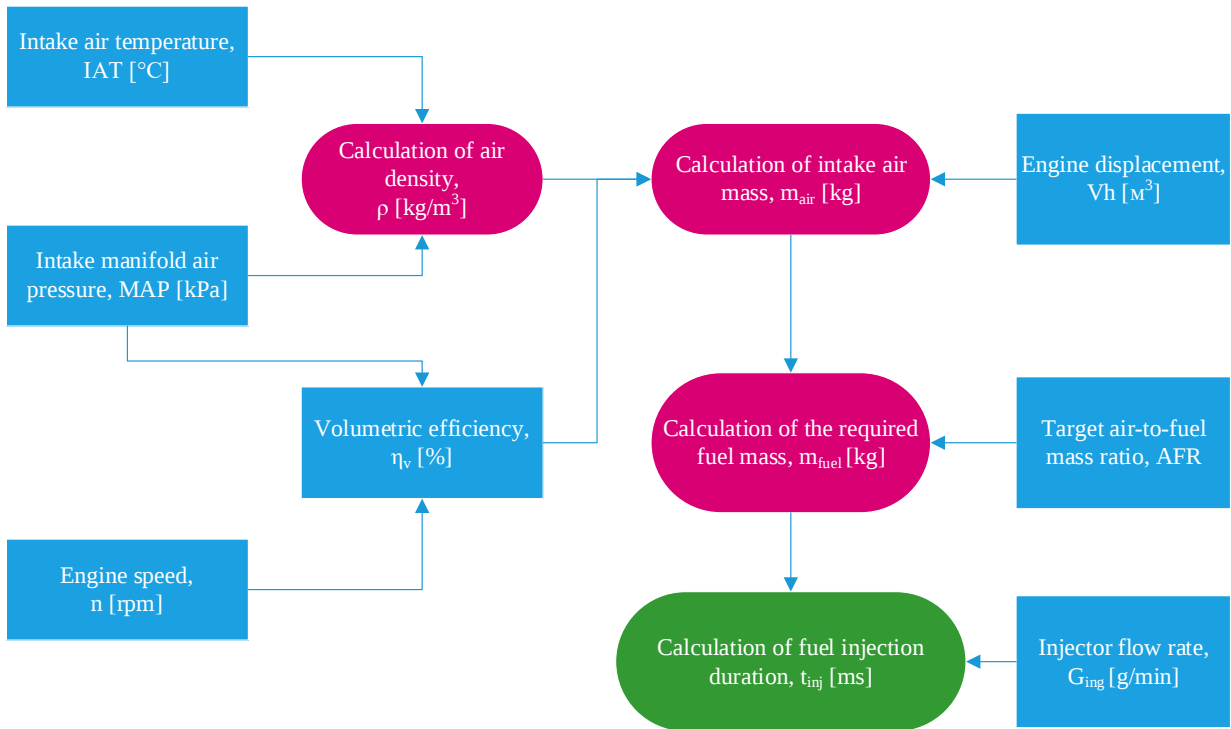
Fig. 2. Speed Density algorithm for calculating the required fuel quantity
