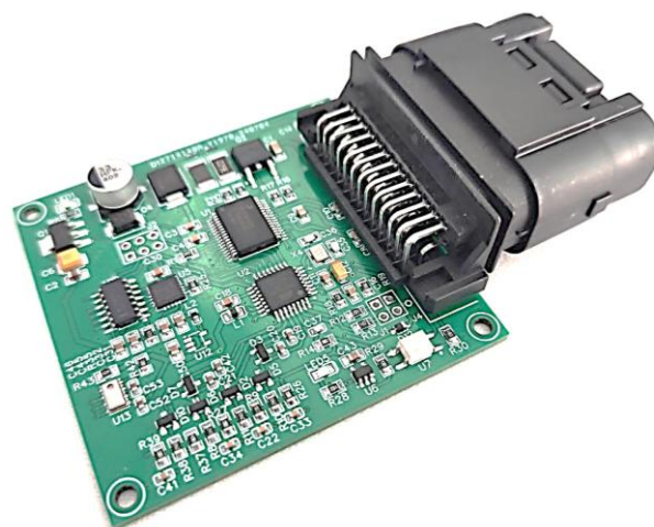
Fig. 6. External view of the developed printed circuit board design for the fuel injection control unit
