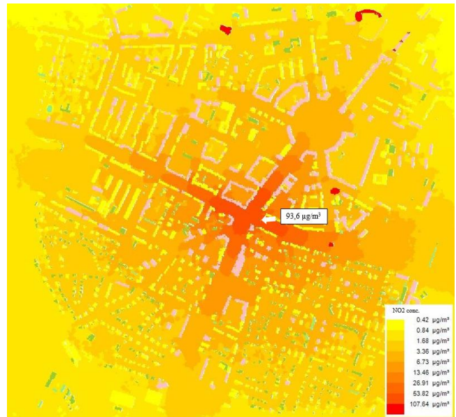
Fig. 8. NO 2 dispersion results for fleet 2
