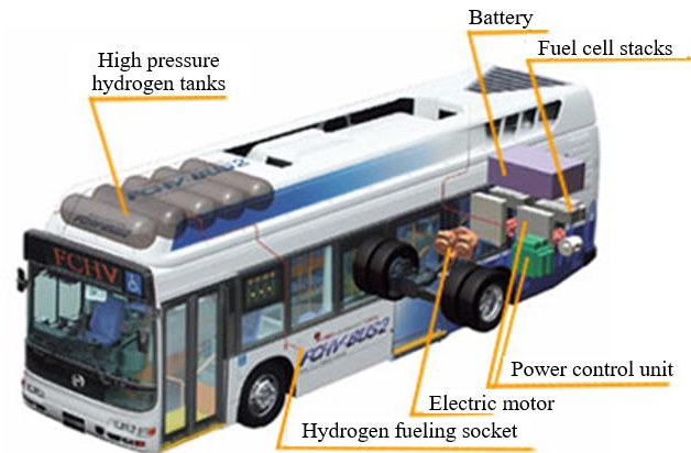
Fig. 1. The propulsion system components of Toyota FCHV-BUS [25]
