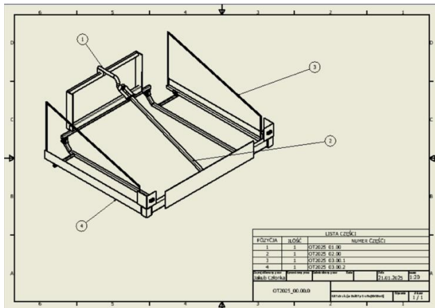
Fig. 14. Assembly diagram of the cover structure
