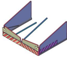
Fig. 2. Conceptual model of transport cover for grain corn harvesting attachment (folded)
