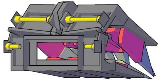
Fig. 5. Model of grain corn harvesting attachment (transport position)
