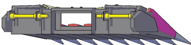
Fig. 4. Model of grain corn harvester attachment (unfolded)
