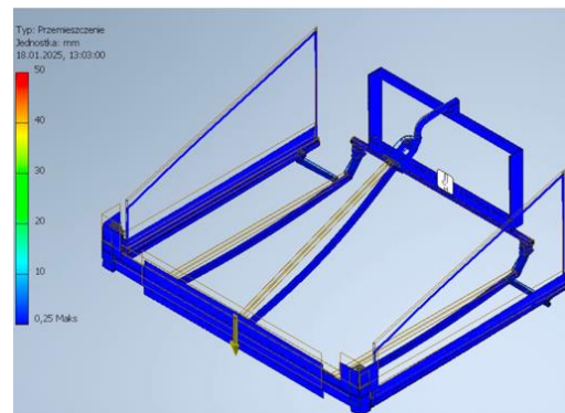
Fig. 13. Displacement of elements – gravity
