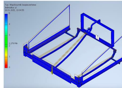
Fig. 12. Safety factor – gravity
