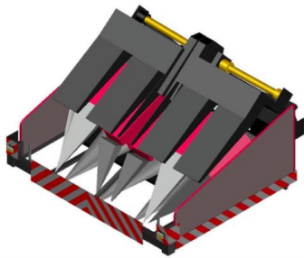
Fig. 8. Model of transport cover hooked on the header (transport position)
