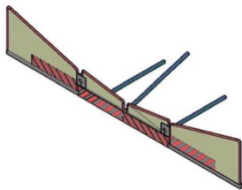
Fig. 3. Conceptual model of transport cover for grain corn harvesting attachment (unfolded)
