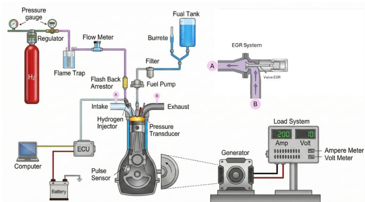
Fig. 1. Experimental setup
