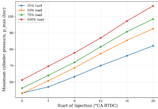
Fig. 5. Variation of maximum cylinder pressure with injection timing at different engine loads (2000 rpm)
