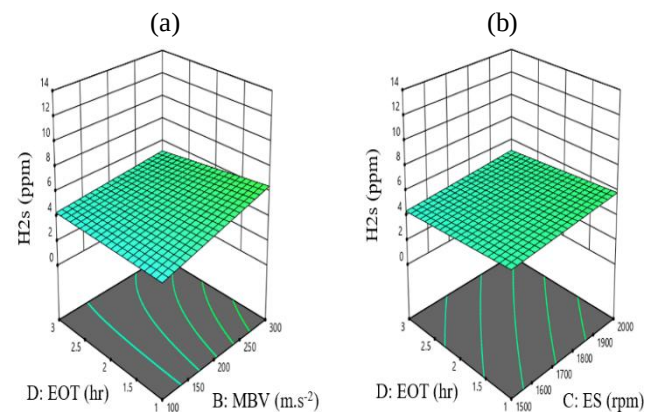
Fig. 11. Variation of \text{H}_2\text{S} emissions against EOT, MBV, and ES: a) the effect of interactions between EOT and MBV on \text{H}_2\text{S} emissions; b) the effect of interactions between EOT and ES on \text{H}_2\text{S} emissions
