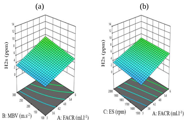
Fig. 9. Variation of \text{H}_2\text{S} emissions against FACR, MBV, and ES: a) the effect of interactions between MBV and FACR on \text{H}_2\text{S} emissions b) the effect of interactions between ES and FACR on \text{H}_2\text{S} emissions
