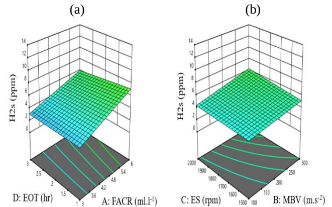
Fig. 10. Variation of \text{H}_2\text{S} emissions against EOT, FACR, ES, and MBV: a) the effect of interactions between EOT and FACR on \text{H}_2\text{S} emissions; b) the effect of interactions between ES and MBV on \text{H}_2\text{S} emissions
